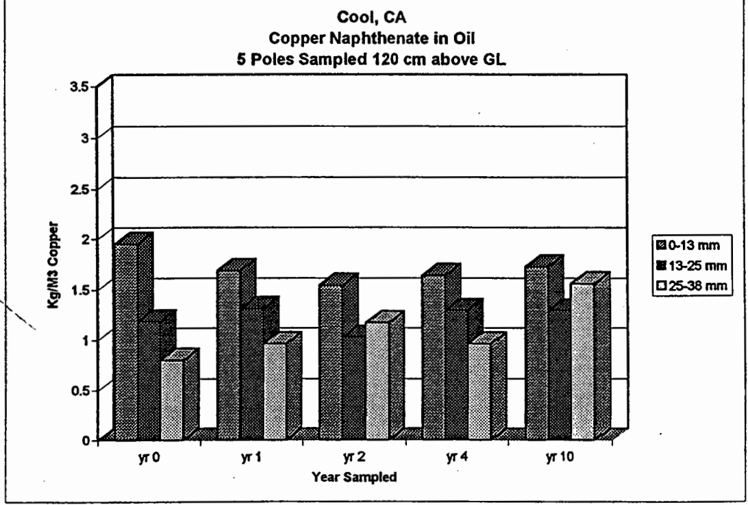
Figure V-11. Copper levels a) 30 or b) 120 cm above the groundline at selected distances from the wood surface of copper naphthenate-treated Douglas-fir poles 0 to 10 years after installation in Cool, California.
