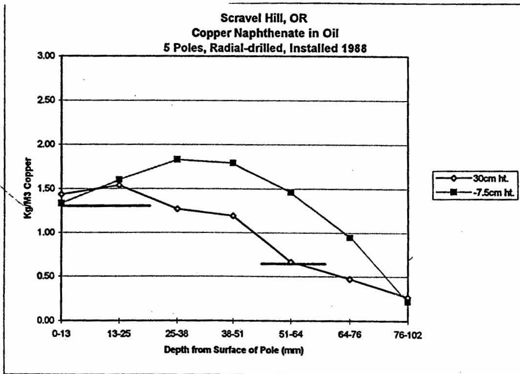
Figure V-4. Copper levels at selected depths in five radially-drilled copper naphthenate-treated Douglas-fir poles 10 years after installation in Scrael Hill, Oregon.
