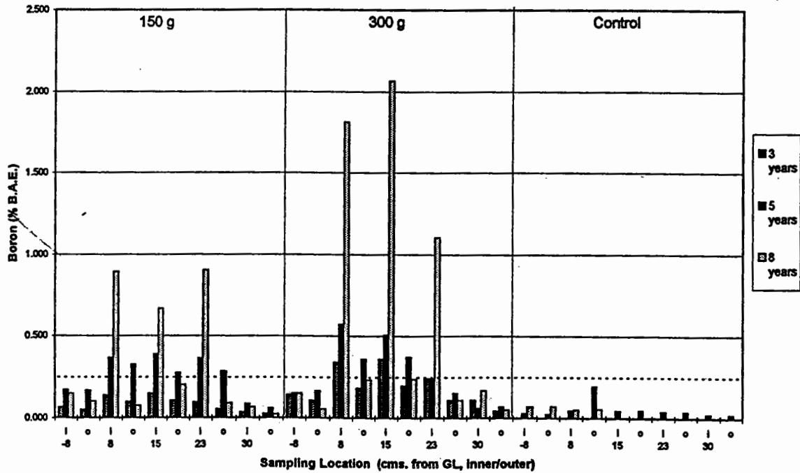
Figure I-7. Residual boron in Douglas-fir poles 3 to 8 years after application of a copper naphthenate/boron paste.
