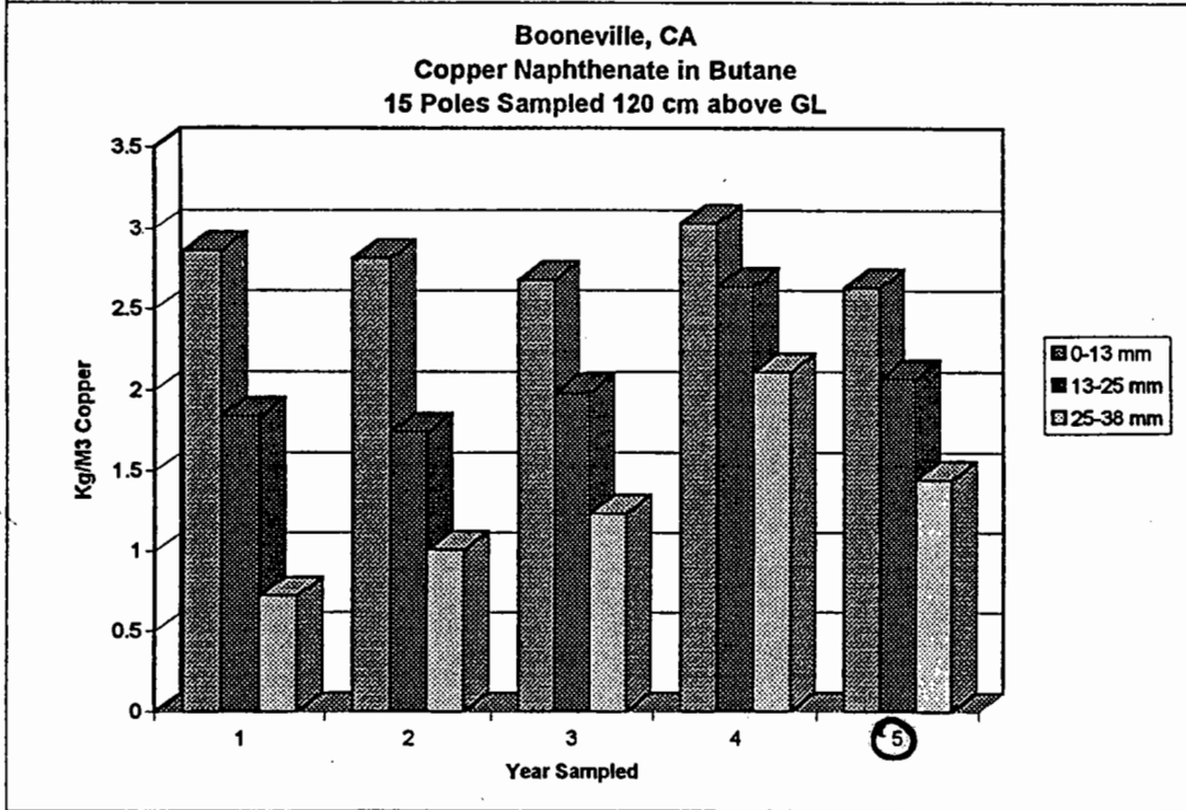
Figure V-12. Copper levels a) 30 or b) 120 cm above the groundline at selected distances from the wood surface of copper naphthenate treated Douglas-fir poles 0 to 10 years after installation in Booneville, California.
