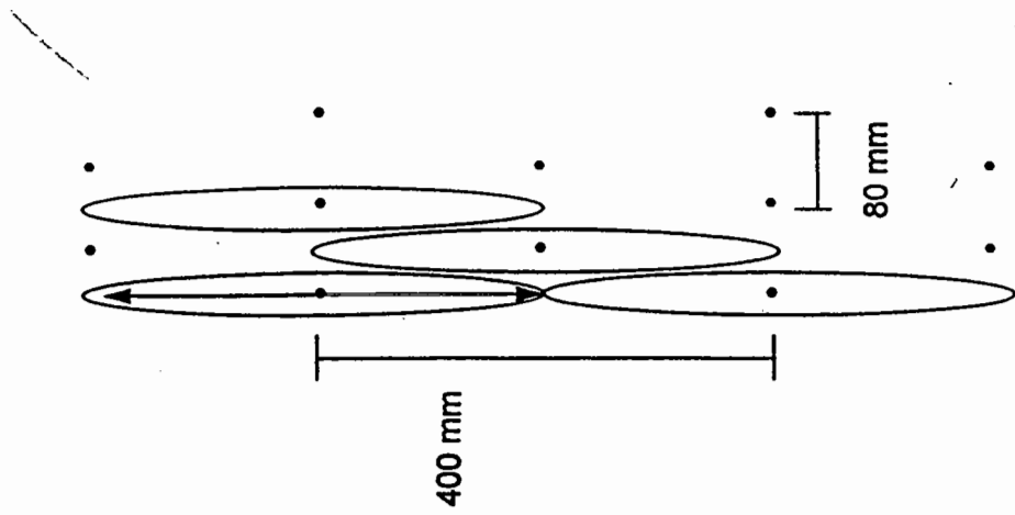
Figure III-2. Possible 400 m longitudinal spacing for through-boring holes to provide average coverage of pole cross section.
